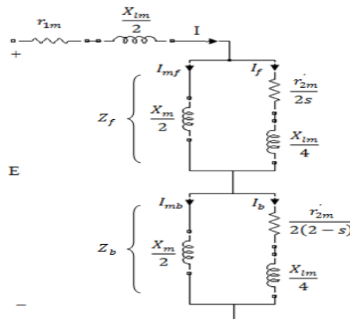
Fig. 1. equivalent circuit of SPIM based on double revolving field theory.
