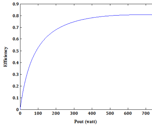
Fig. 4. Variation of designed motor efficiency against output power.
