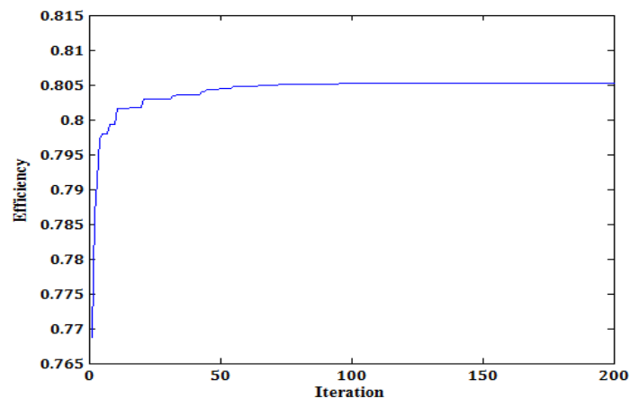
Fig. 3. Variation of efficiency against PSO iteration number.
