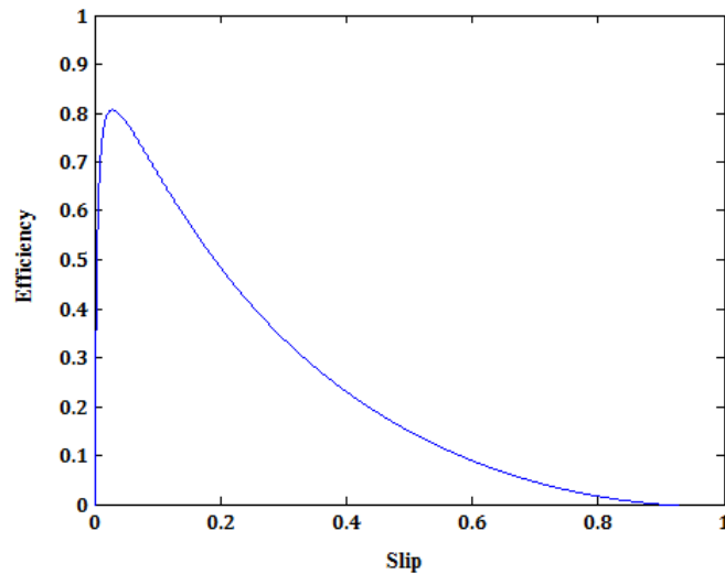
Fig. 5. Variation of motor efficiency against rotor slip.
