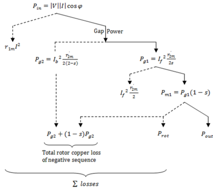
Fig. 2. power flow diagram for a SPIM.
